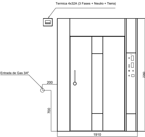
VISTA FRONTAL
